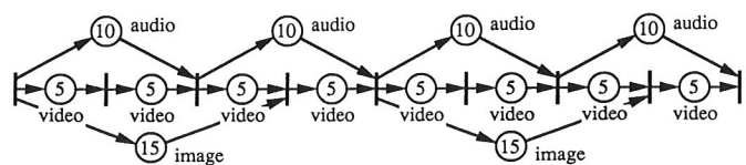
Figure 7. Audio, video and image OCPN timing specification
