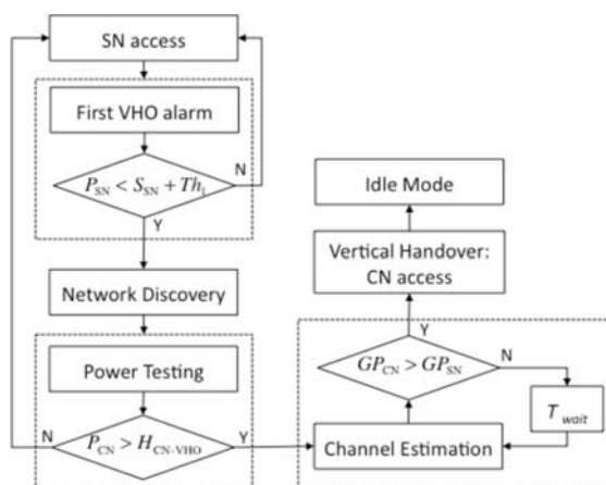
Figure 2.17: Decision tree for RSS-VHDF approach.
