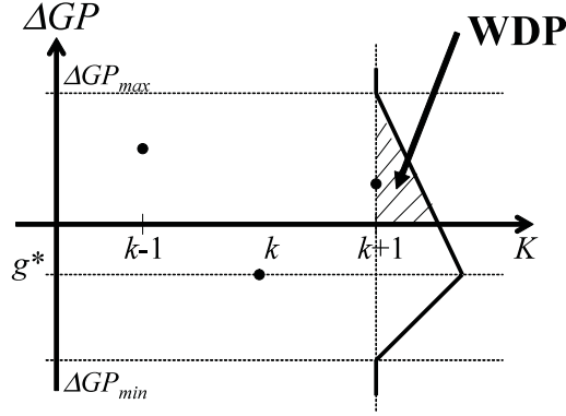
Figure 2.23: WDP profile for g^* < 0 case.
