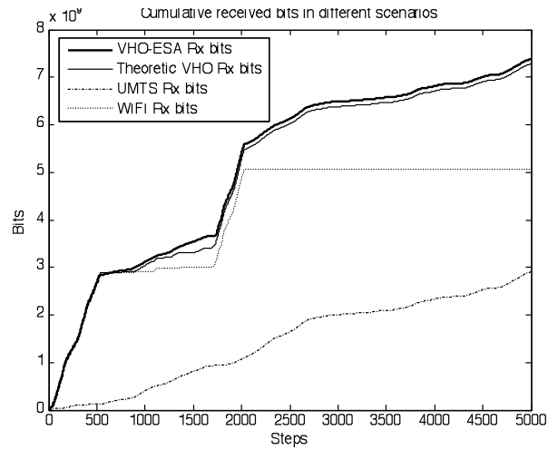
Figure 2.9: Performance of the proposed VHO algorithm, [1].
