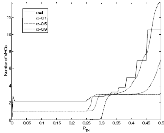
Figure 2.26: Number of vertical handovers vs. P_{TH} .
