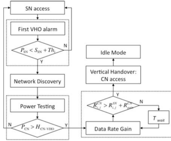
Figure 2.19: Decision tree for C-VHDF approach.
