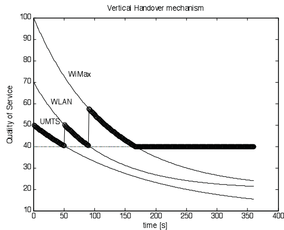
Figure 2.4: Theoretical behaviour of QoS-based VHO algorithm.
