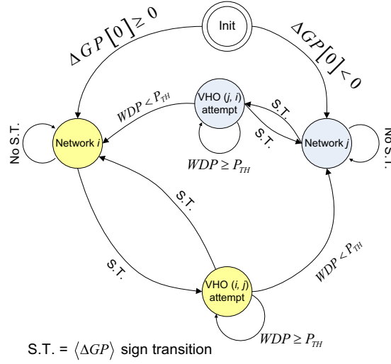
Figure 2.24: VHO Algorithm Finite State Machine.
