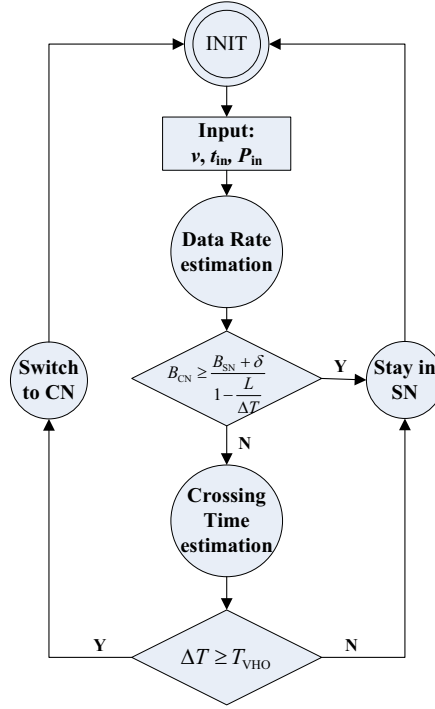
Figure 2.28: Speed Vertical Handover (S-VHO) algorithm.
