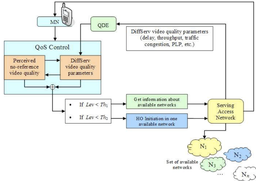
Figure 2.3: Proposed network architecture for QoS-based handoff.
