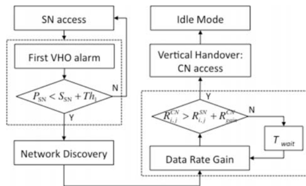
Figure 2.18: Decision tree for DR-VHDF approach.
