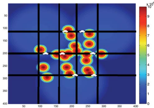
Figure 2.29: Vertical handover simulated scenario for vehicular environment.
