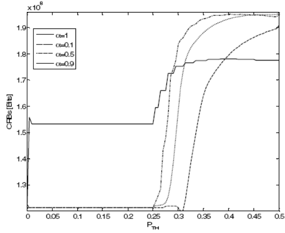
Figure 2.25: Cumulative Received Bits vs. P_{TH} .
