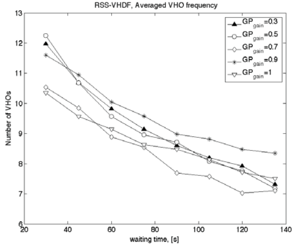
Figure 2.22: Average VHO frequency for RSS-VHDF.
