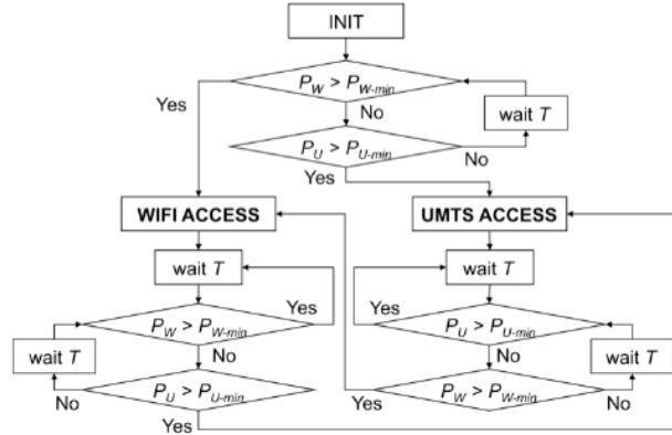
Figure 2.15: PB-VHO Flowchart.
