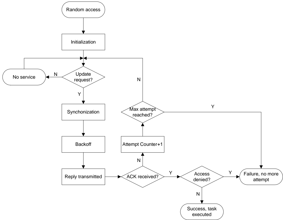
Figure 4-14: New user device's access flow chart
