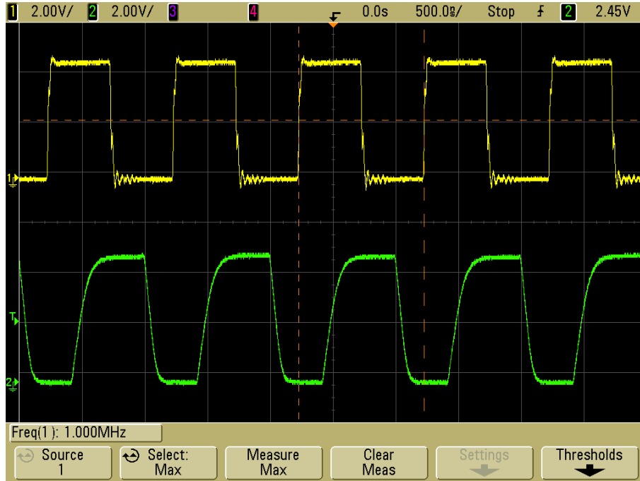
Figure 3-8: Waveforms of transmit and receive signals [WCL11]
