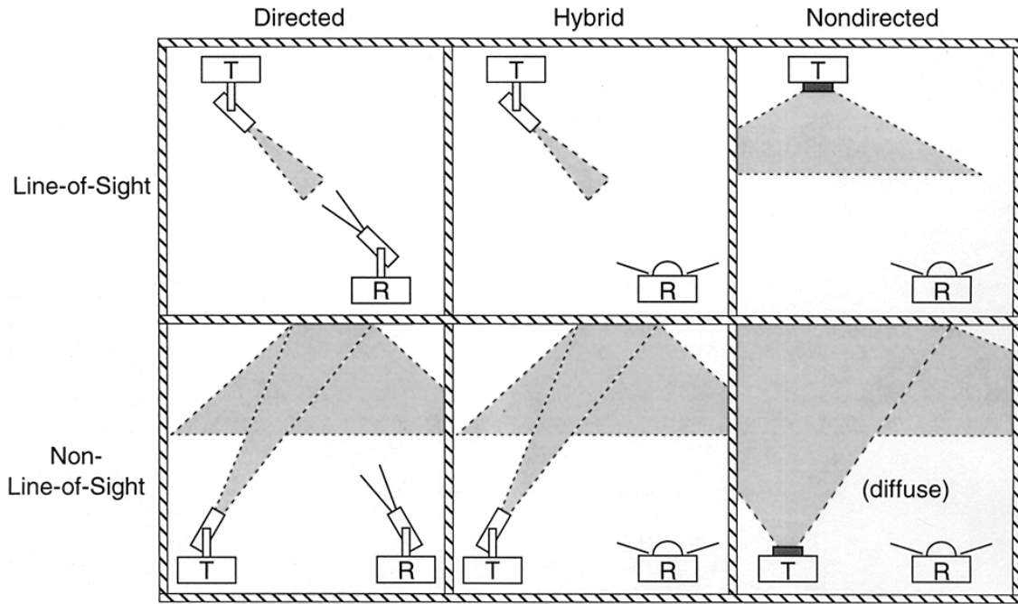
Figure 2-1: Classification of simple links according to the degree of directionality of the transmitter and receiver and whether the link relies upon the existence of a LOS path between them [KB97]
