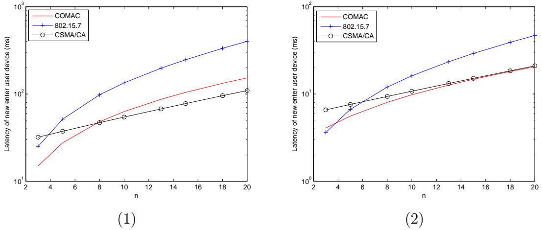
Figure 4-16: Latency comparison with rate of (1) 1 Mb/s and (2) 10 Mb/s for CSMA/CA, COMAC and 802.15.7 standard
