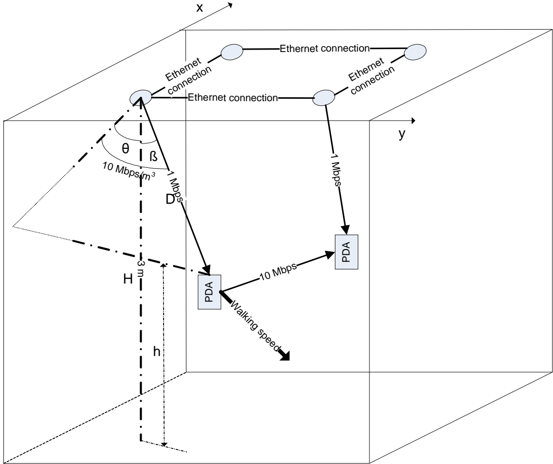
Figure 3-2: Proposed FSO system model for indoor applications
