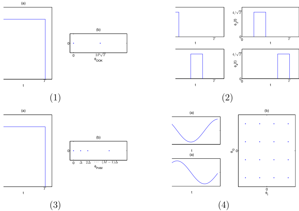
Figure 2-5: Basis function (a) and Constellation of Symbols (b) for (1)OOK, (2)4-PPM, (3)PAM and (4)QAM
