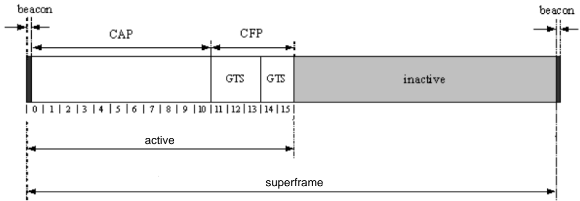
Figure 4-12: An example of the superframe structure [oEG11]
