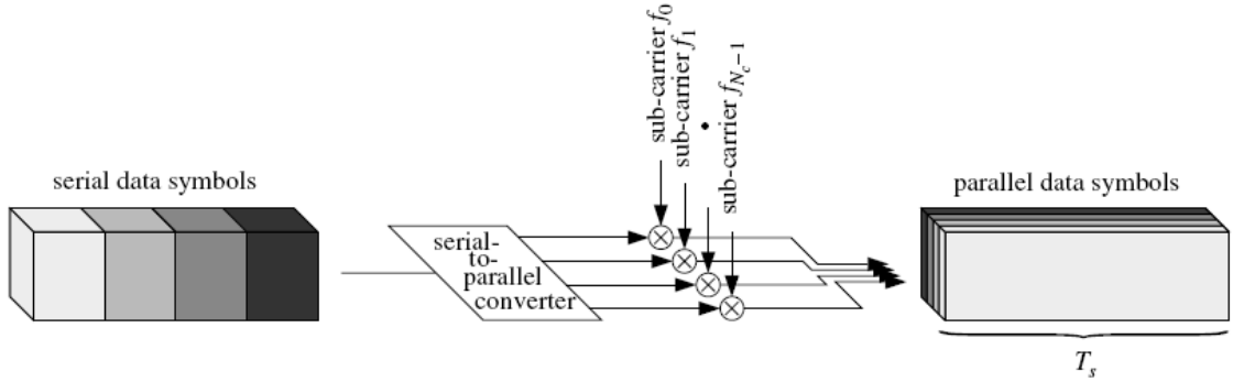
Figure 3-9: Orthogonal Frequency Division Multiplexing [FK03]
