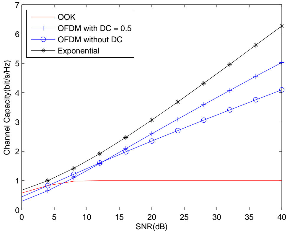
Figure 3-12: Channel capacities for four different cases under unit average power constraint
