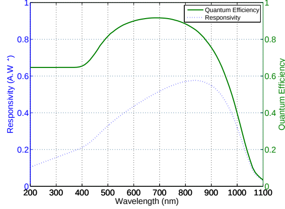
Figure 4: Receiver quantum efficiency and responsivity [16]
