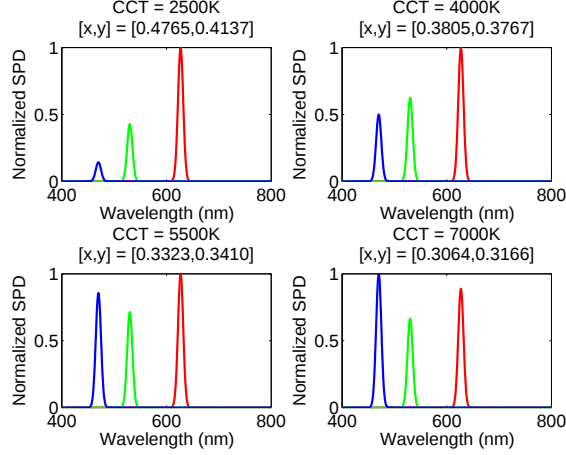
Figure 2: Transmitting element normalized spectral power distribution
