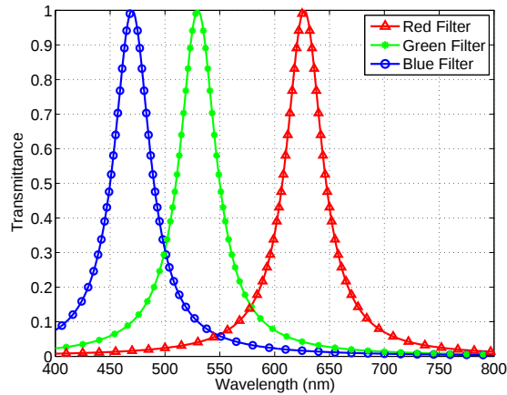
Figure 3: Filter transmittance for full width at half maximum = 40nm
