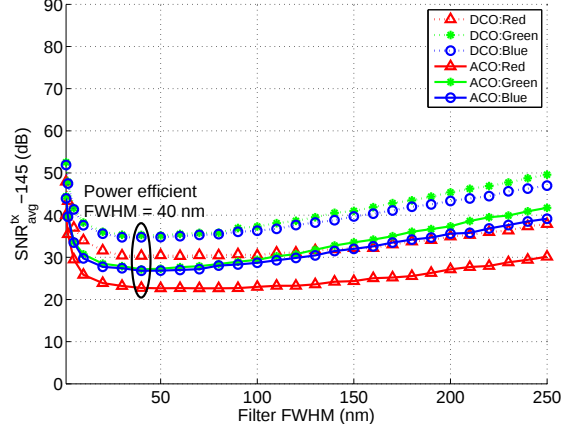
Figure 7: \text{SNR}_{\text{avg}}^{\text{tx}} vs filter full width at half maximum to achieve \text{BER} \leq 10^{-3} Transmitter: \sigma_r = \sigma_g = \sigma_b = 5 \text{ nm} ; CCT = 6250 K
