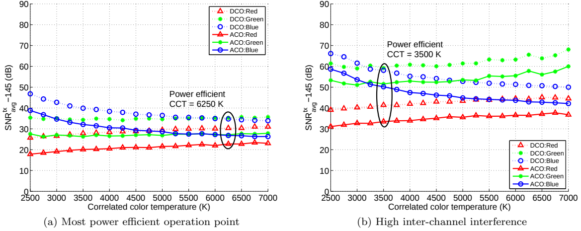
Figure 5: \text{SNR}_{\text{avg}}^{\text{tx}} vs correlated color temperature to achieve \text{BER} \leq 10^{-3}
