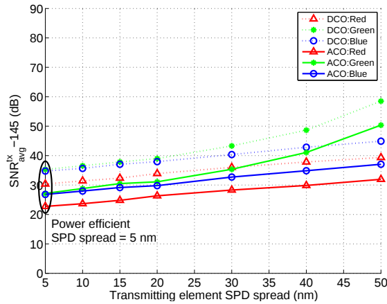
Figure 6: \text{SNR}_{\text{avg}}^{\text{tx}} vs transmitting element spectral power distribution spread to achieve \text{BER} \leq 10^{-3}
