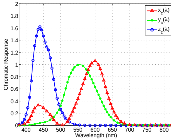
Figure 1: CIE XYZ 1931 model color matching functions
